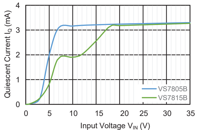
Quiescent Current
