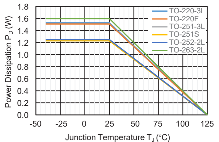
Power Dissipation
