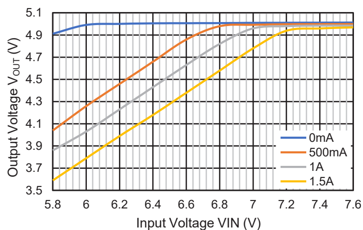
VS7805E Dropout Voltage
