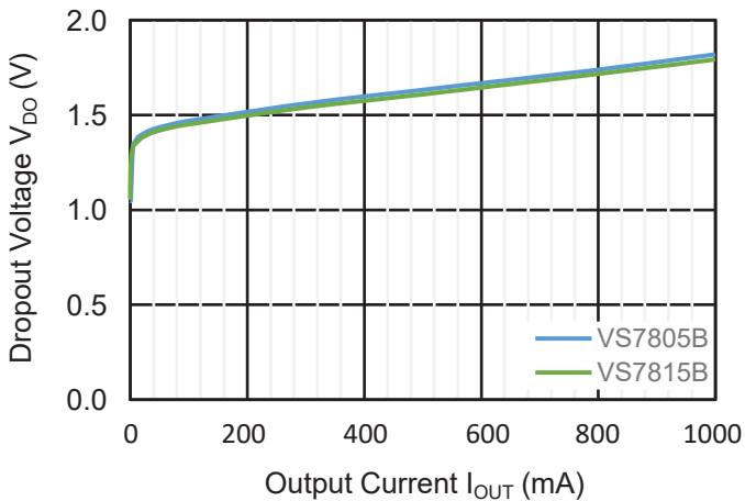
Dropout Voltage
