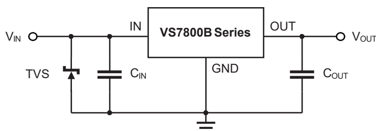
Figure 9-4. TVS is used at IN
