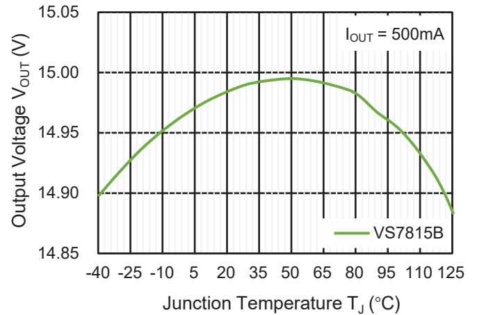
Temperature Characteristics
