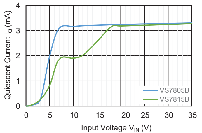
Quiescent Current
