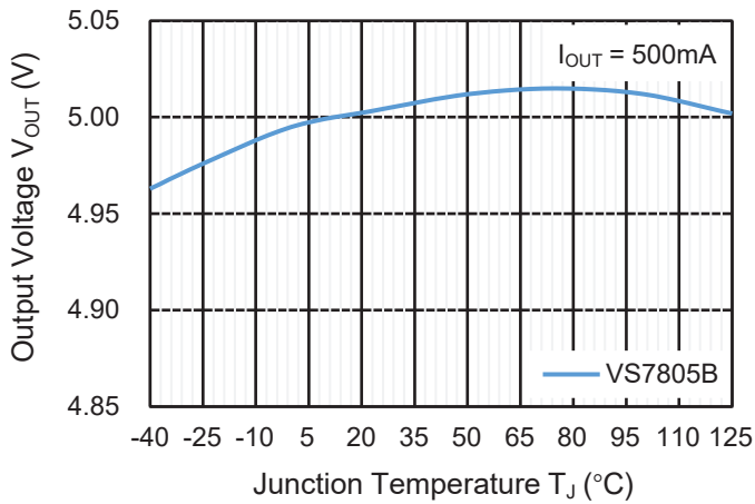
Temperature Characteristics
