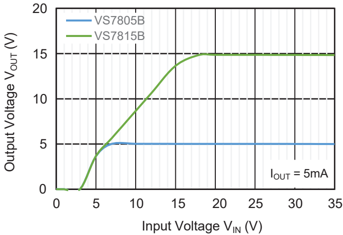
Line Regulation
