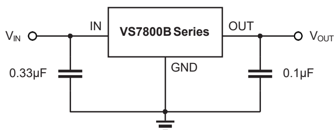
Figure 9-3. Conventional Circuit
