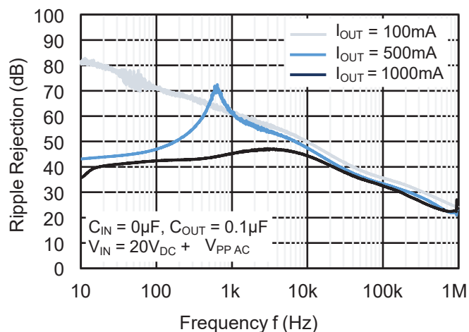
Ripple Rejection
