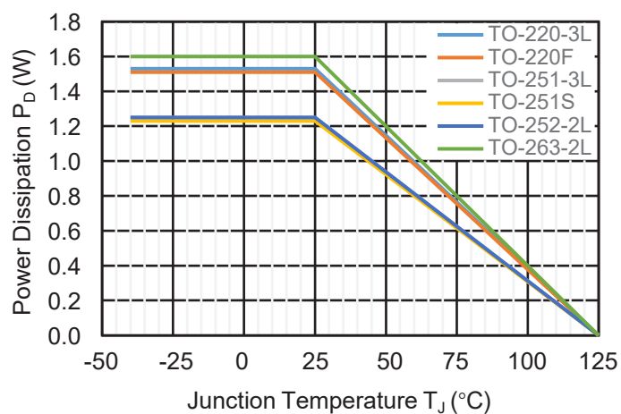
Power Dissipation
