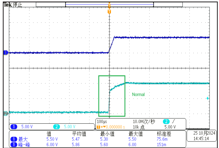
Figure 9-2. Test with the circuit that a 100µF/25V electrolytic capacitor parallel to the C_{IN} [Test Circuit is shown in Figure 9-6]
