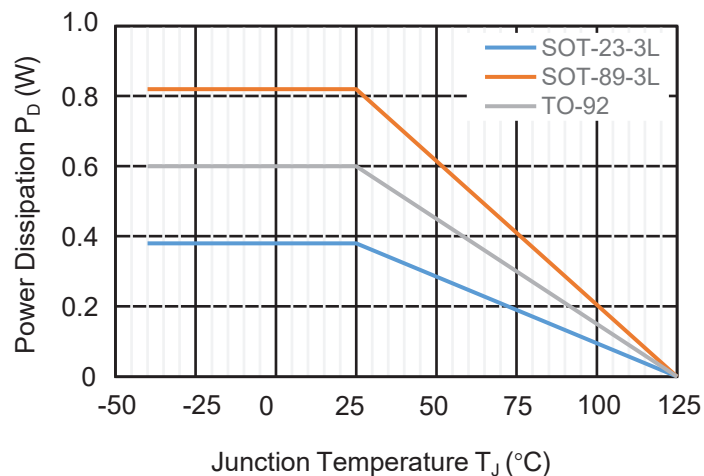
Power Dissipation
