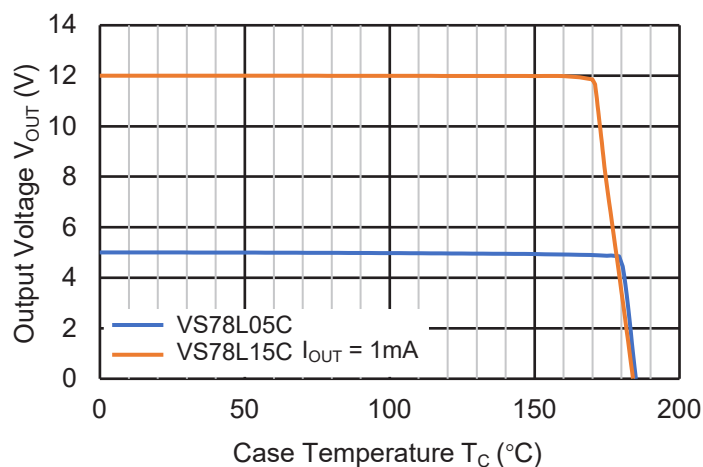
Thermal Shutdown
