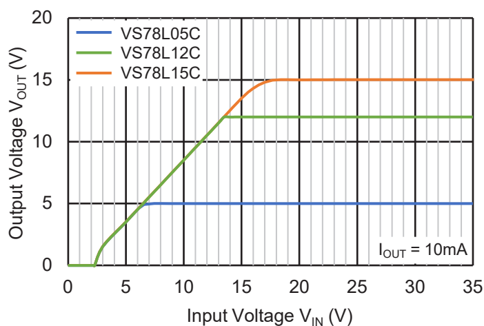
Line Regulation
