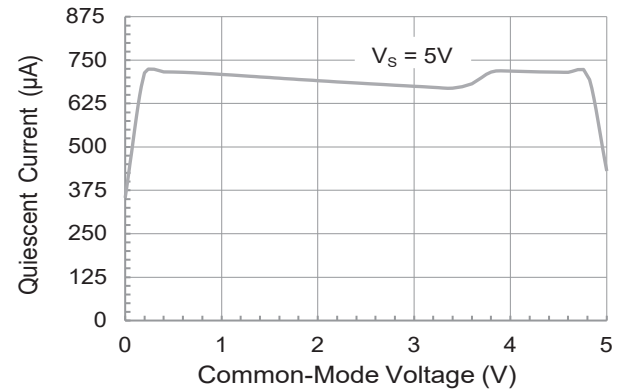
Quiescent Current vs. Input Common-mode Voltage
